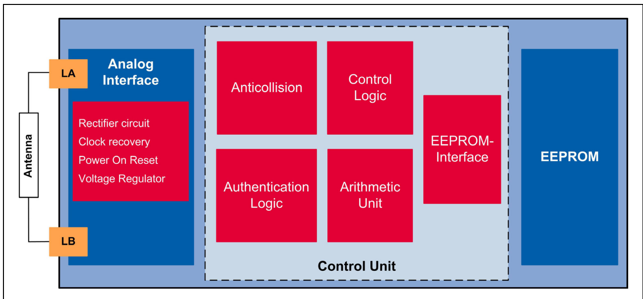
Figure 5 Block Diagram
